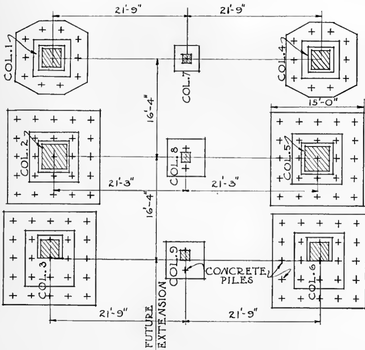
SECTION A-A. FOOTING PLAN
